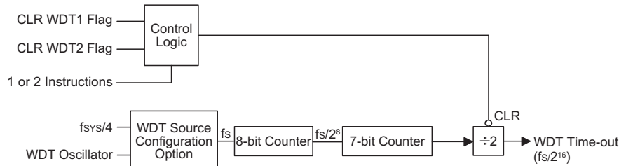
Watchdog Timer
