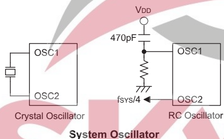
System Oscillator
